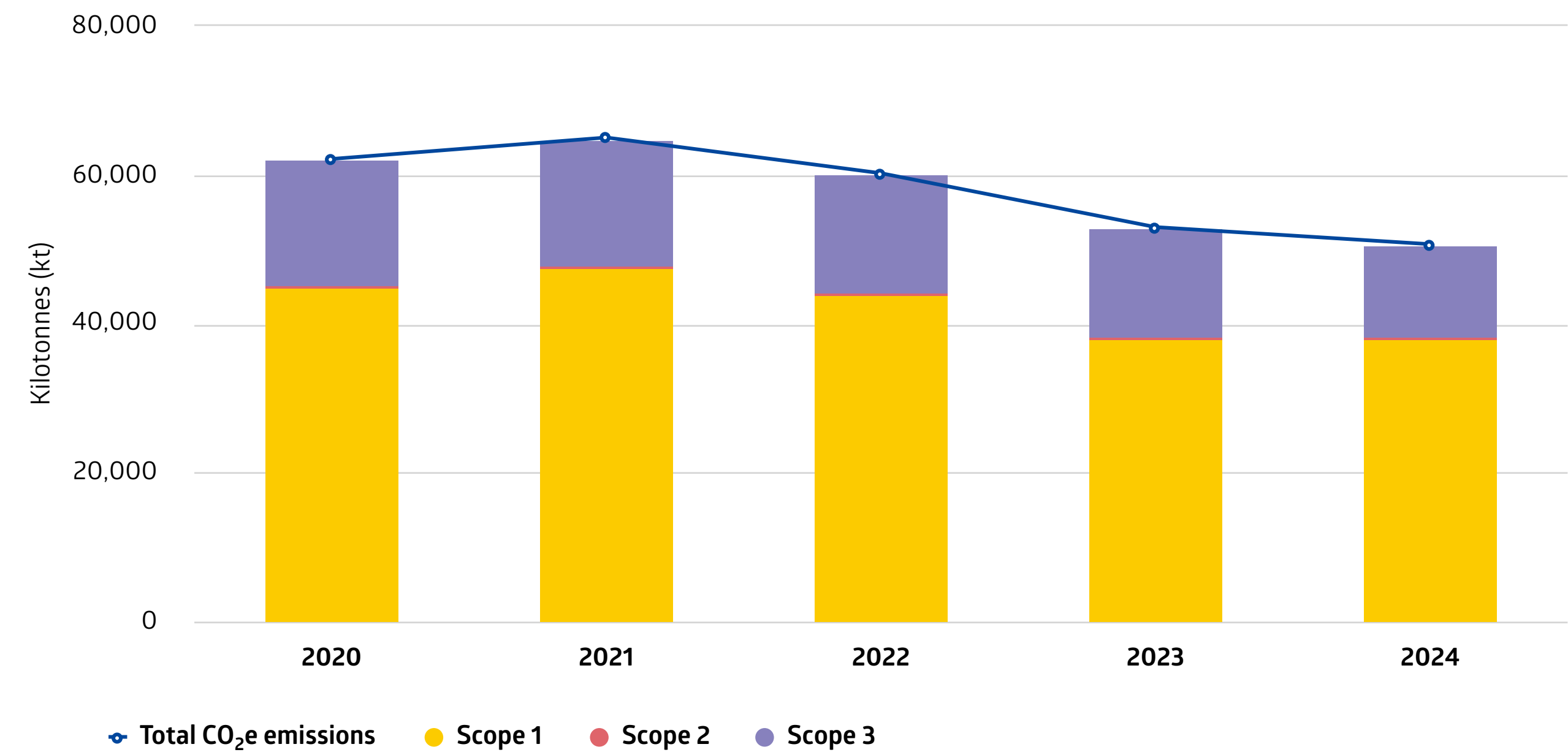
Total CO 2 e emissions - on an equity basis
